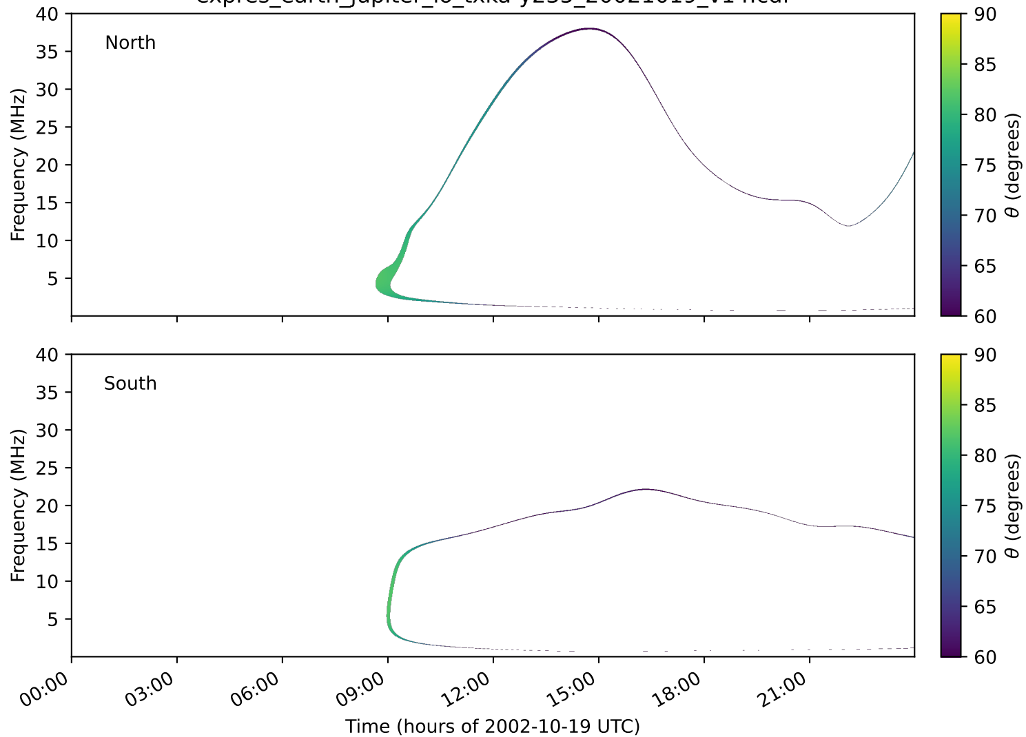
expres_earth_jupiter_io_txka-y235_20021019_v14.cdf
