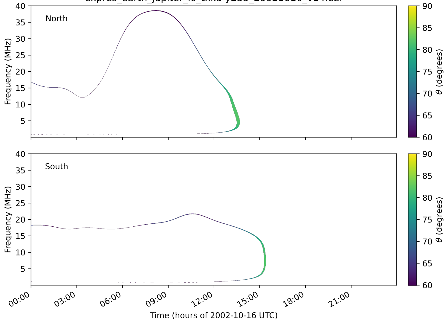
expres_earth_jupiter_io_txka-y235_20021016_v14.cdf
