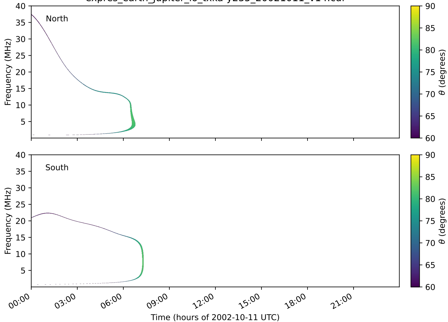
expres_earth_jupiter_io_txka-y235_20021011_v14.cdf
