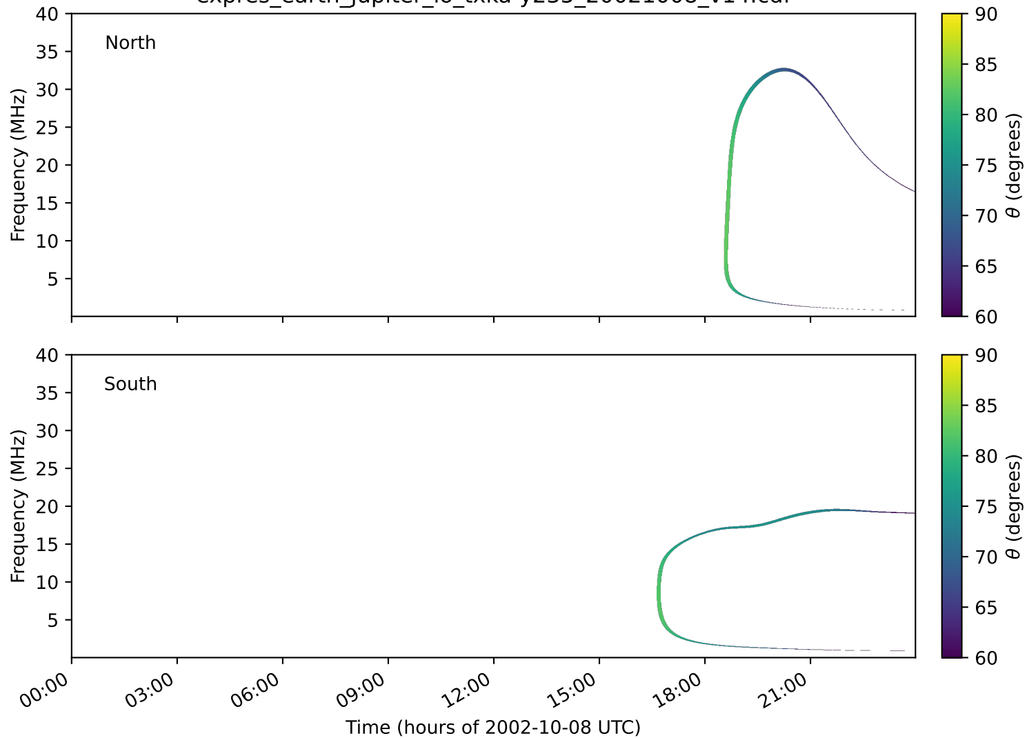
expres_earth_jupiter_io_txka-y235_20021008_v14.cdf
