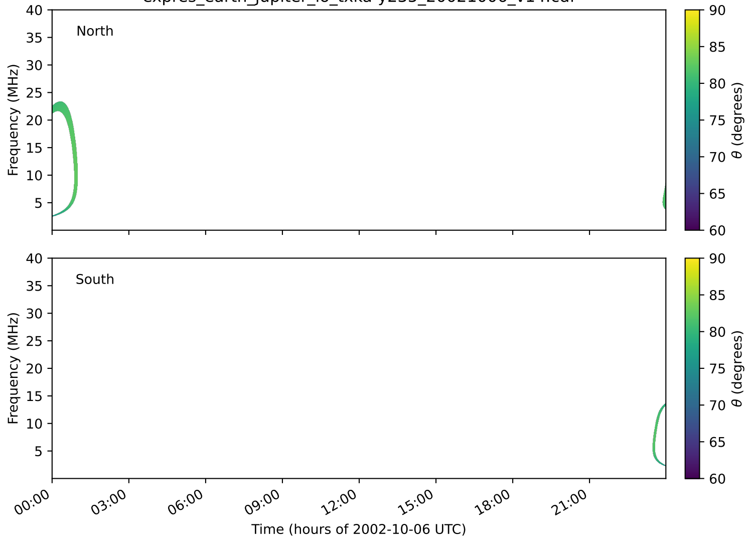
expres_earth_jupiter_io_txka-y235_20021006_v14.cdf
