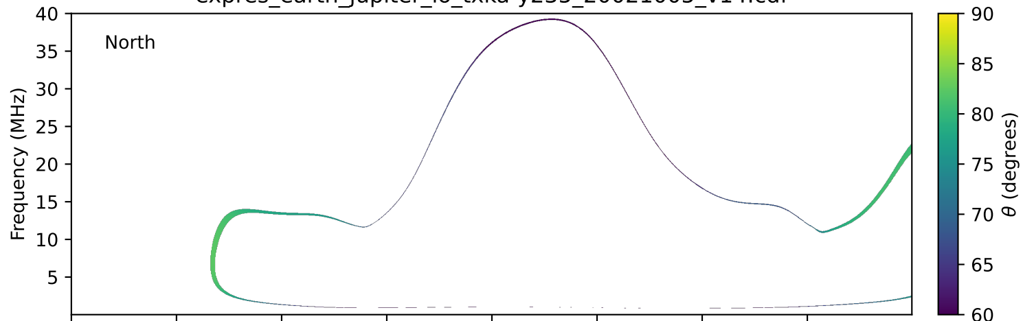
expres_earth_jupiter_io_txka-y235_20021005_v14.cdf
