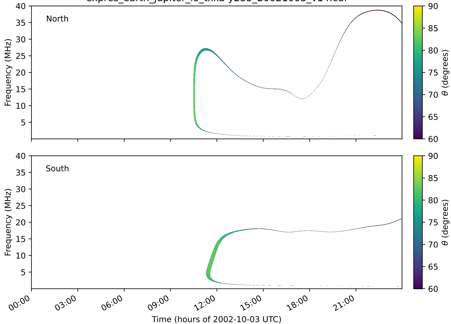
expres_earth_jupiter_io_txka-y235_20021003_v14.cdf
