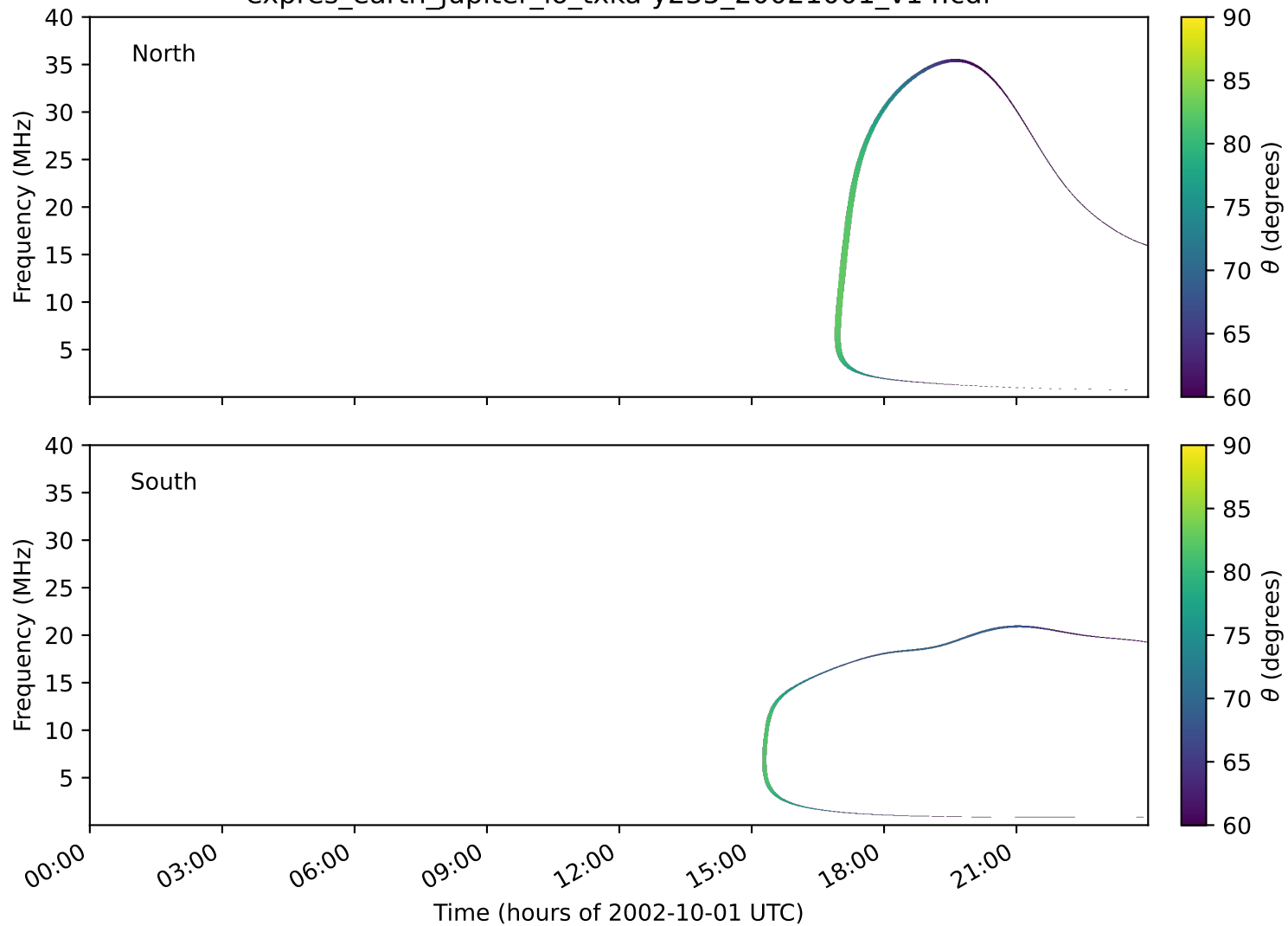
expres_earth_jupiter_io_txka-y235_20021001_v14.cdf
