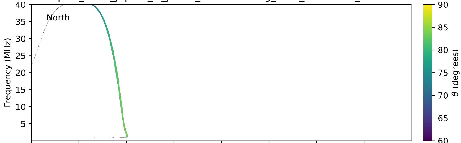
expres_earth_jupiter_io_jrm33_lossc-wid1deg_3kev_20021027_v11.cdf
