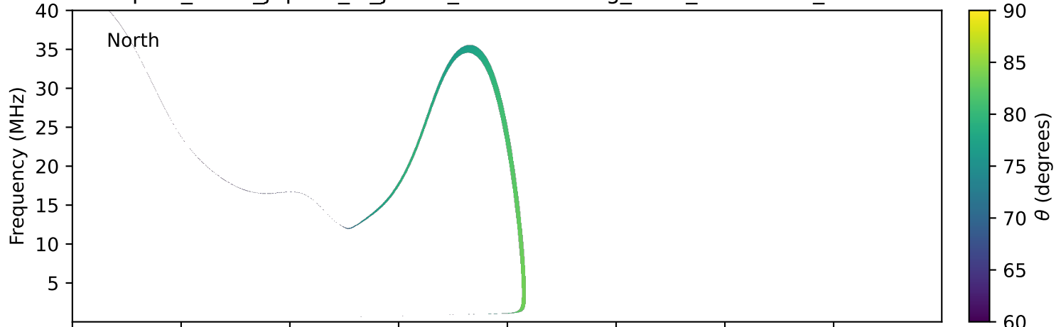
expres_earth_jupiter_io_jrm33_lossc-wid1deg_3kev_20021025_v11.cdf
