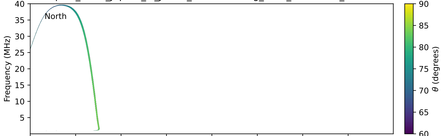
expres_earth_jupiter_io_jrm33_lossc-wid1deg_3kev_20021020_v11.cdf
