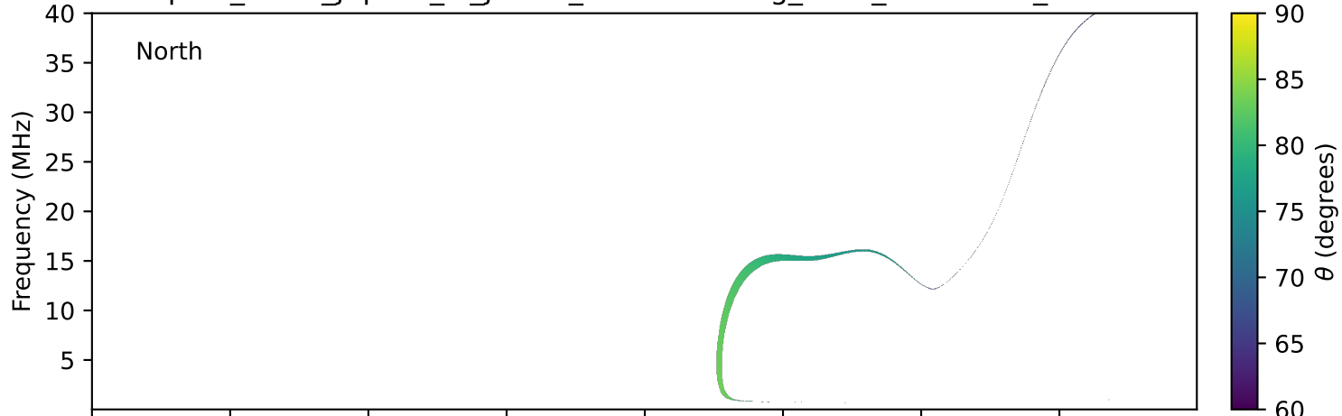
expres_earth_jupiter_io_jrm33_lossc-wid1deg_3kev_20021017_v11.cdf
