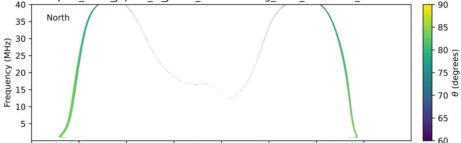
expres_earth_jupiter_io_jrm33_lossc-wid1deg_3kev_20021014_v11.cdf
