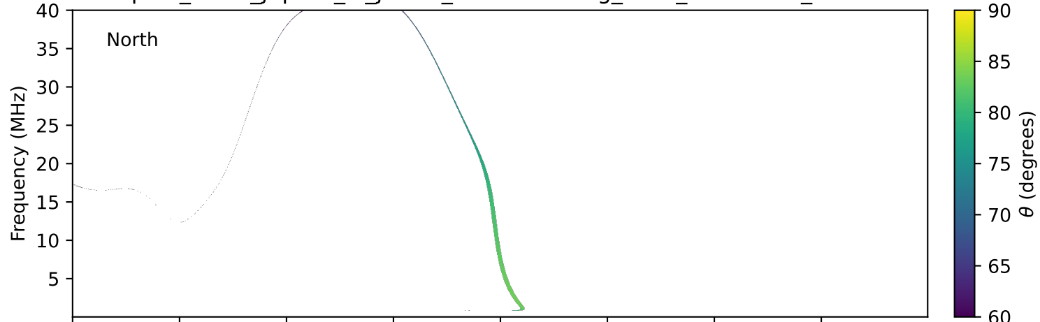
expres_earth_jupiter_io_jrm33_lossc-wid1deg_3kev_20021009_v11.cdf
