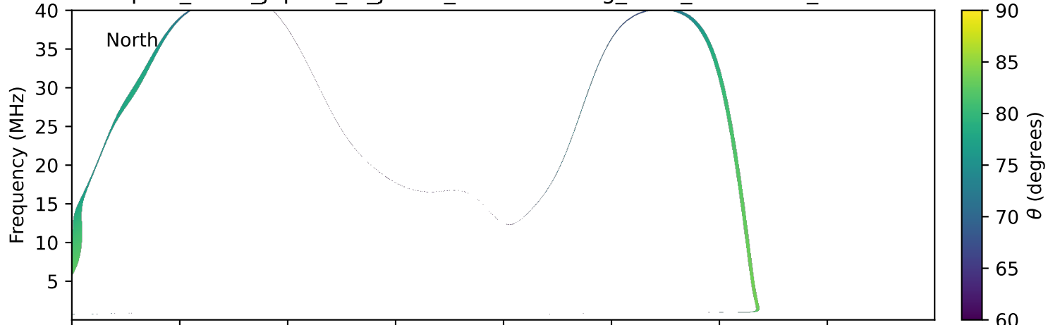
expres_earth_jupiter_io_jrm33_lossc-wid1deg_3kev_20021007_v11.cdf
