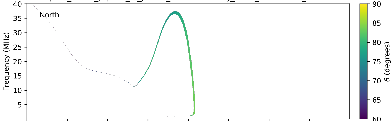
expres_earth_jupiter_io_jrm09_lossc-wid1deg_3kev_20021025_v11.cdf
