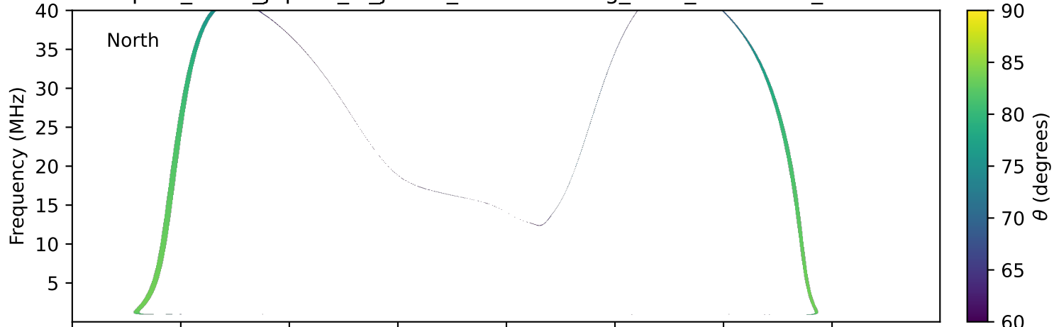
expres_earth_jupiter_io_jrm09_lossc-wid1deg_3kev_20021014_v11.cdf
