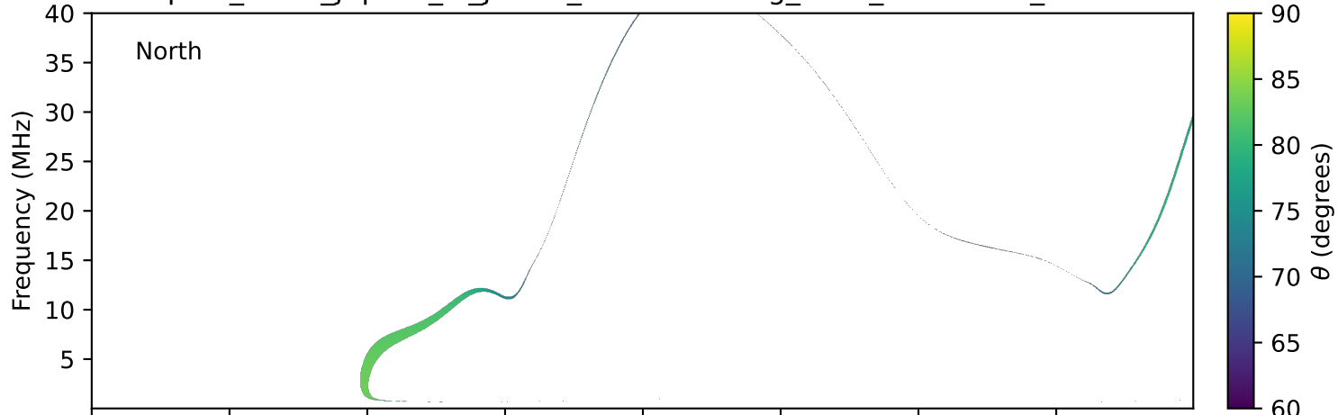
expres_earth_jupiter_io_jrm09_lossc-wid1deg_3kev_20021012_v11.cdf
