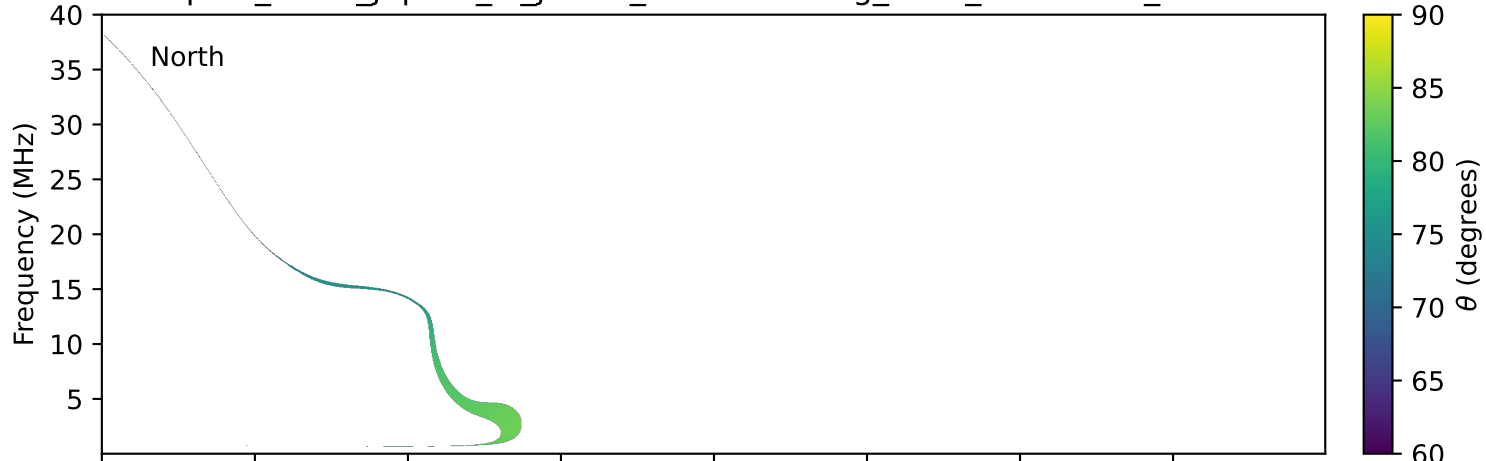
expres_earth_jupiter_io_jrm09_lossc-wid1deg_3kev_20021011_v11.cdf
