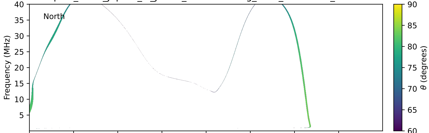
expres_earth_jupiter_io_jrm09_lossc-wid1deg_3kev_20021007_v11.cdf
