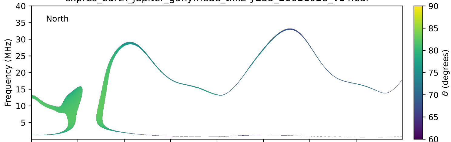
expres_earth_jupiter_ganymede_txka-y235_20021028_v14.cdf
