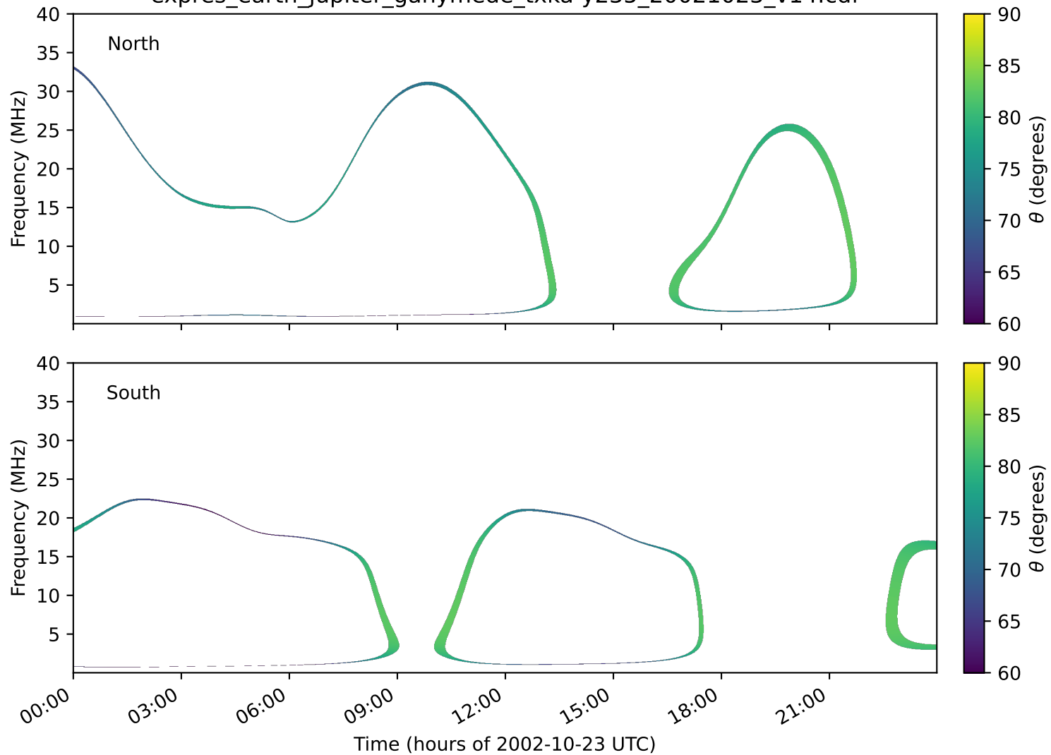
expres_earth_jupiter_ganymede_txka-y235_20021023_v14.cdf
