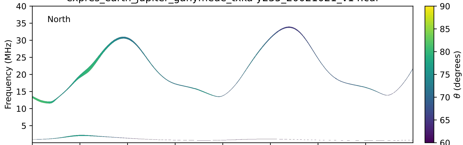
expres_earth_jupiter_ganymede_txka-y235_20021021_v14.cdf
