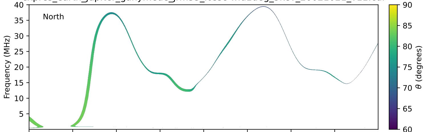
expres_earth_jupiter_ganymede_jrm33_lossc-wid1deg_3kev_20021021_v11.cdf
