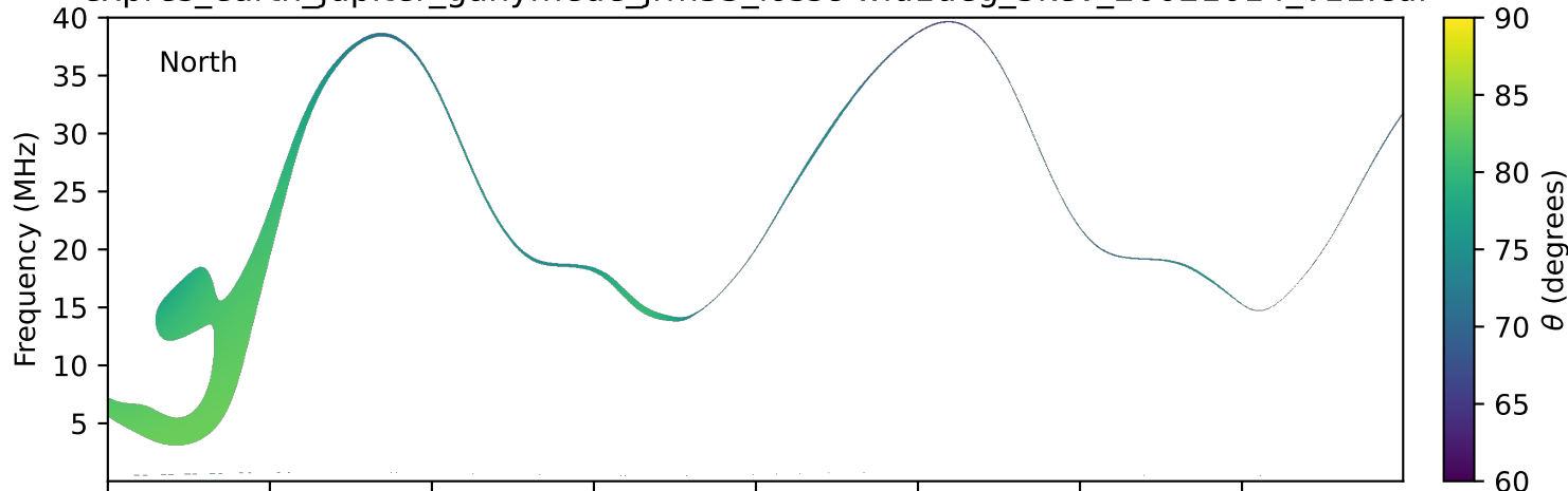
expres_earth_jupiter_ganymede_jrm33_lossc-wid1deg_3kev_20021014_v11.cdf
