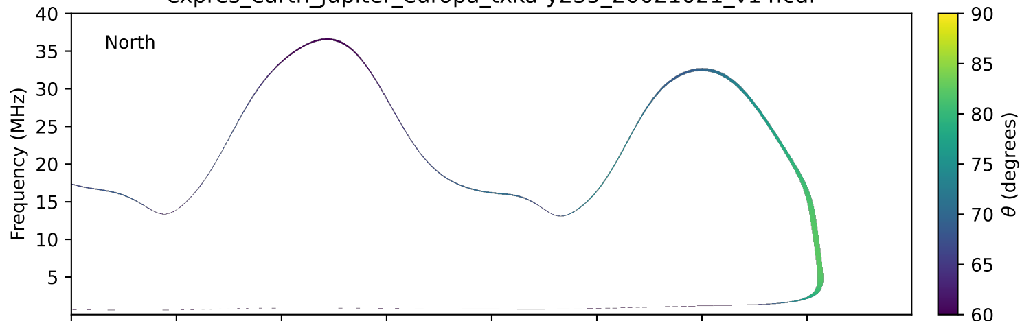
expres_earth_jupiter_europa_txka-y235_20021021_v14.cdf
