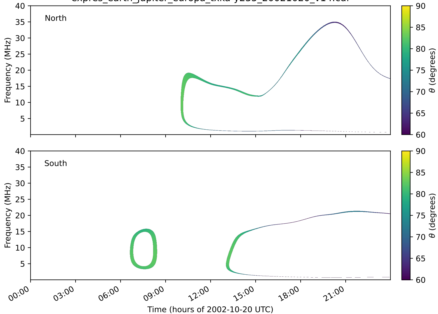
expres_earth_jupiter_europa_txka-y235_20021020_v14.cdf
