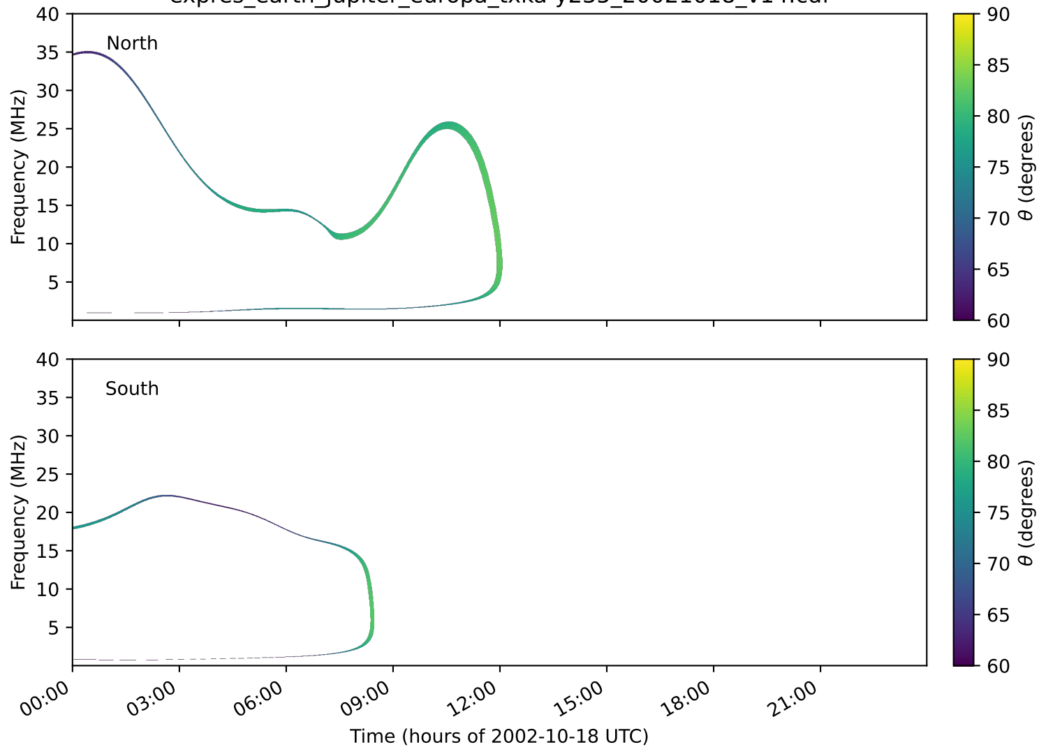
expres_earth_jupiter_europa_txka-y235_20021018_v14.cdf
