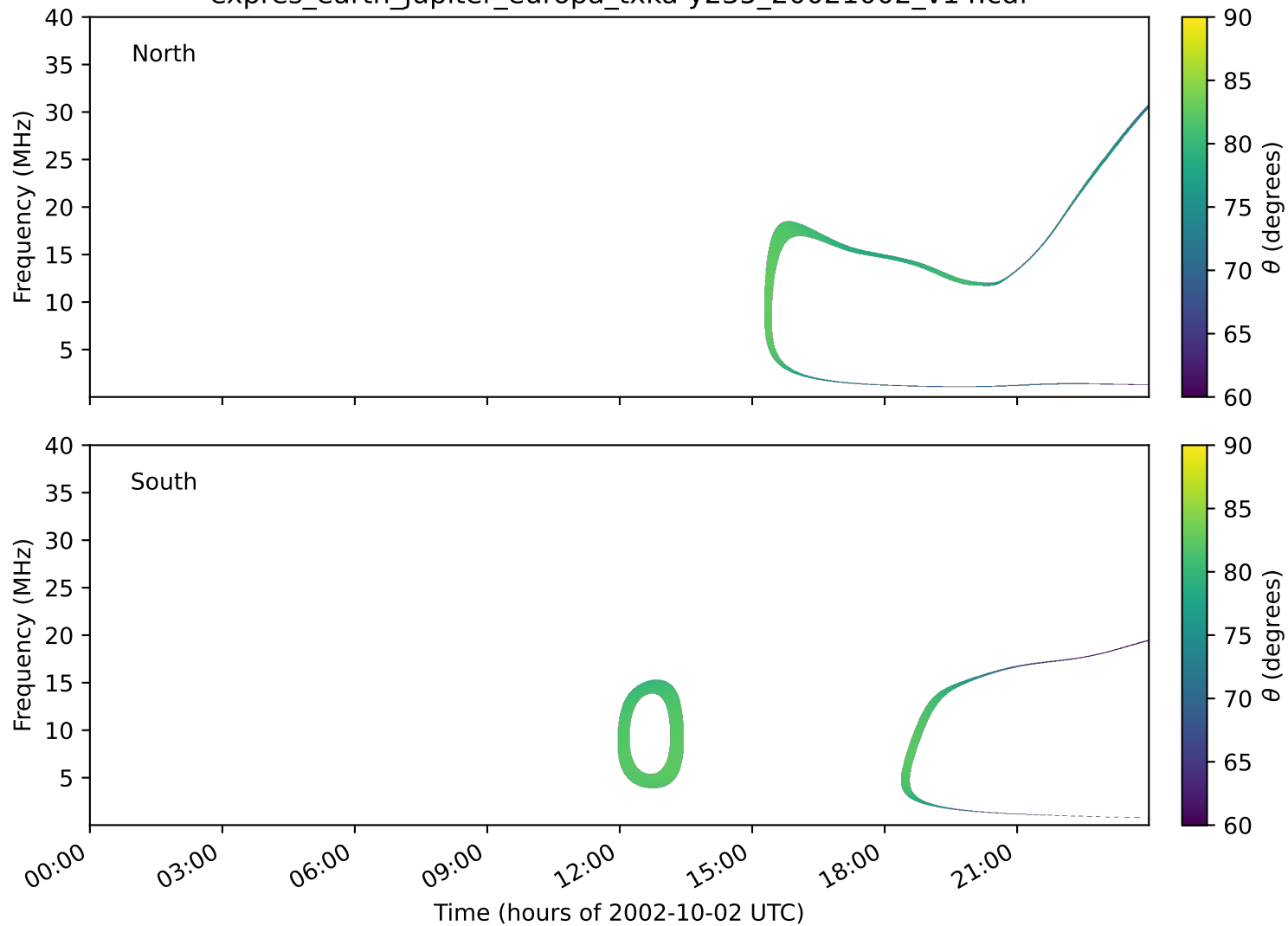
expres_earth_jupiter_europa_txka-y235_20021002_v14.cdf
