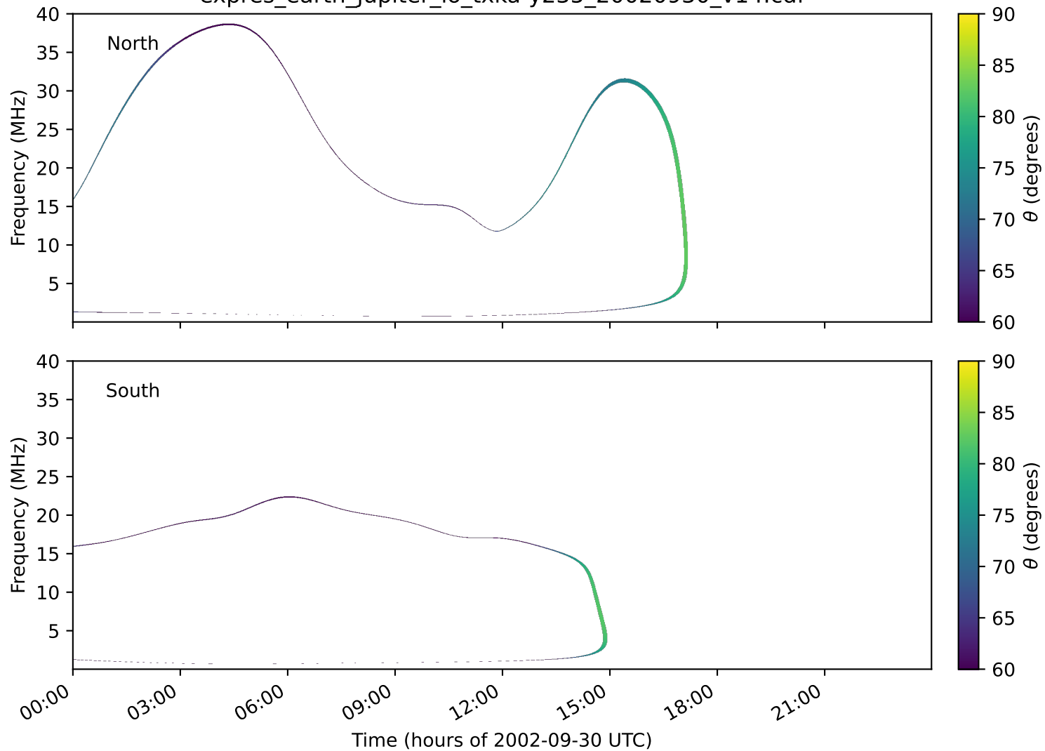
expres_earth_jupiter_io_txka-y235_20020930_v14.cdf
