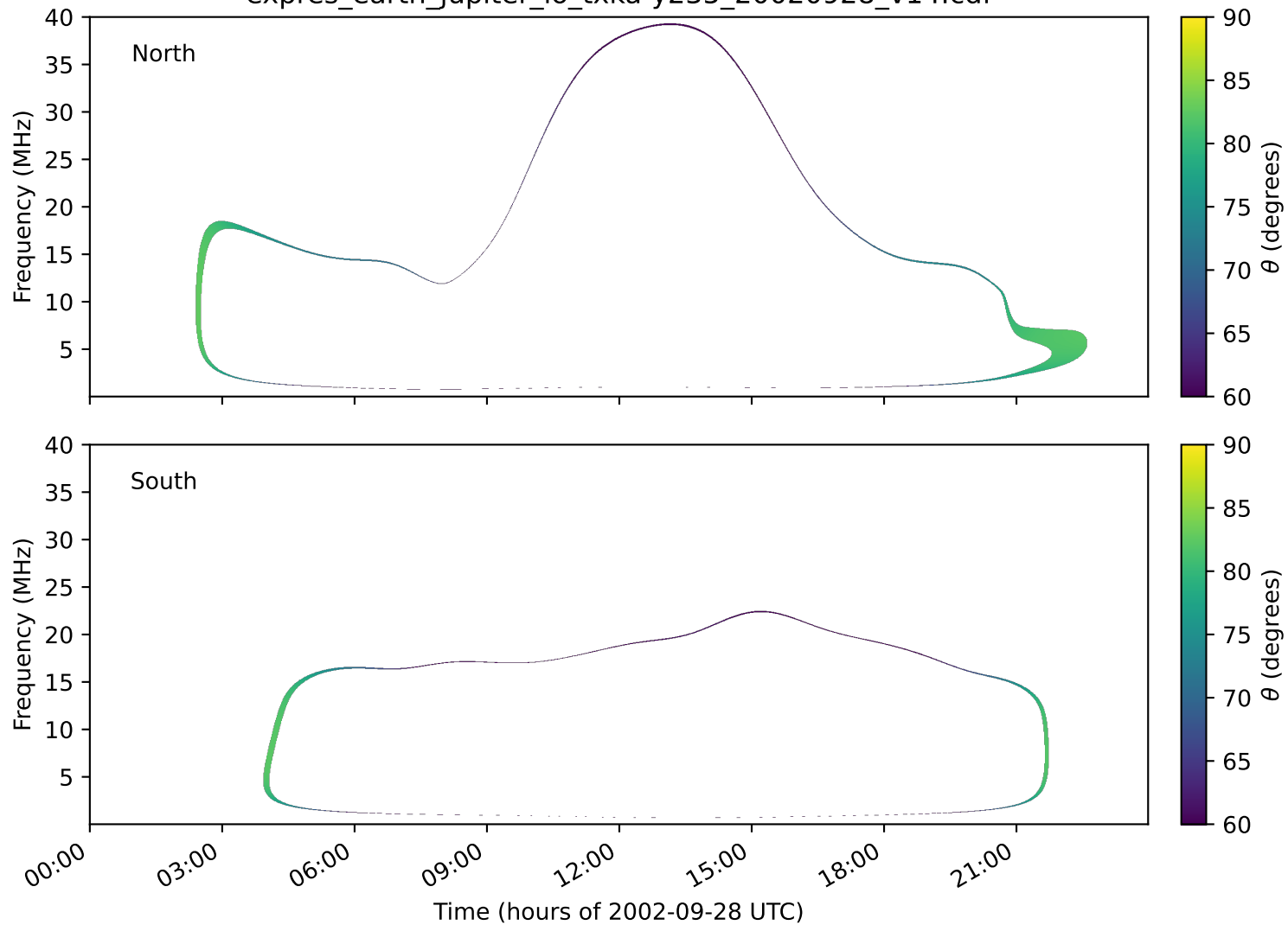
expres_earth_jupiter_io_txka-y235_20020928_v14.cdf
