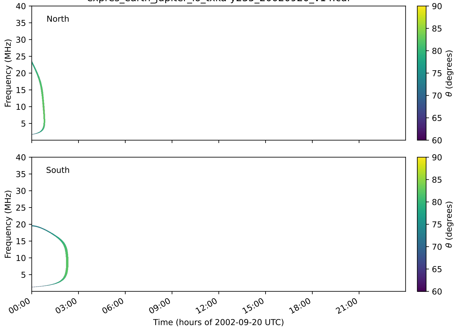
expres_earth_jupiter_io_txka-y235_20020920_v14.cdf
