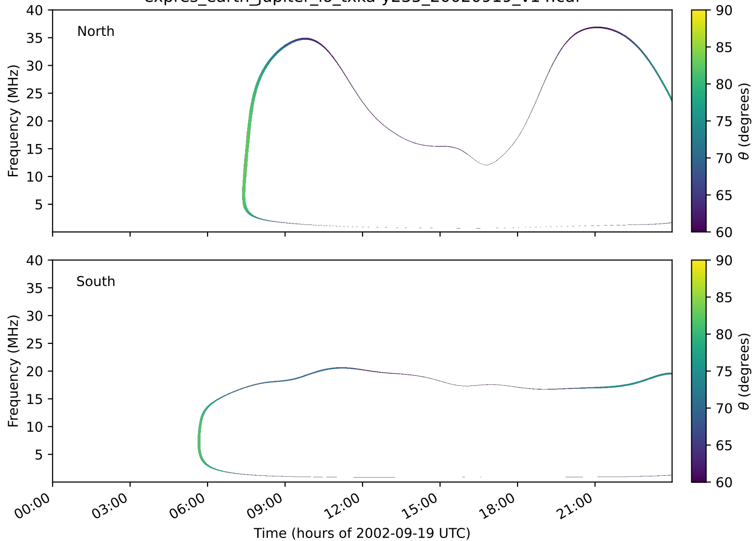
expres_earth_jupiter_io_txka-y235_20020919_v14.cdf
