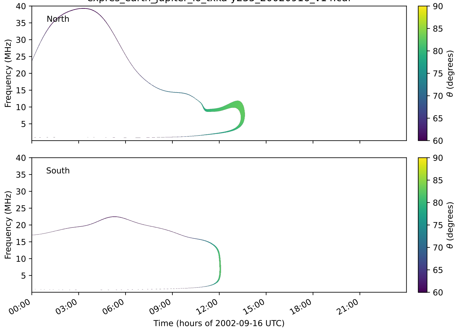
expres_earth_jupiter_io_txka-y235_20020916_v14.cdf
