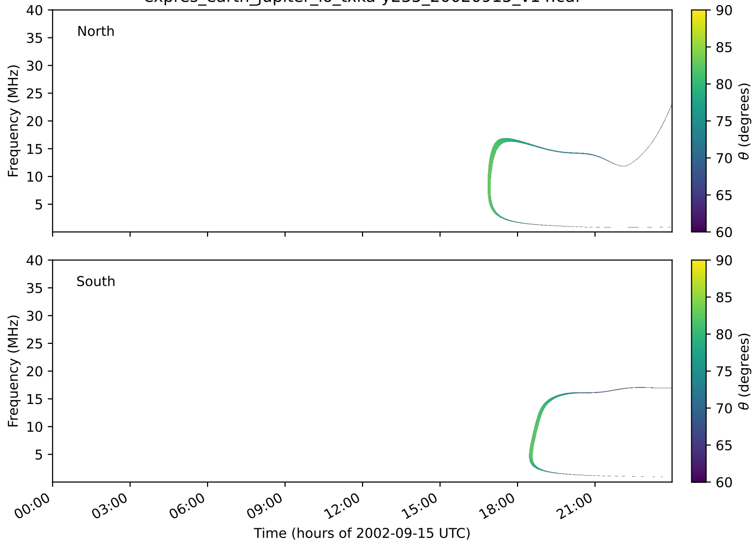
expres_earth_jupiter_io_txka-y235_20020915_v14.cdf
