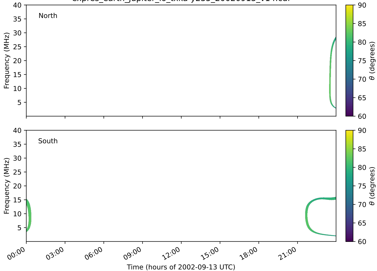
expres_earth_jupiter_io_txka-y235_20020913_v14.cdf
