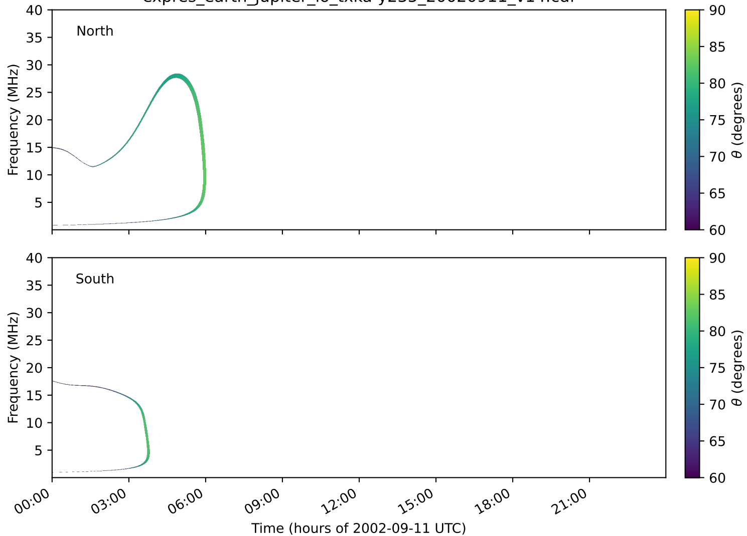
expres_earth_jupiter_io_txka-y235_20020911_v14.cdf
