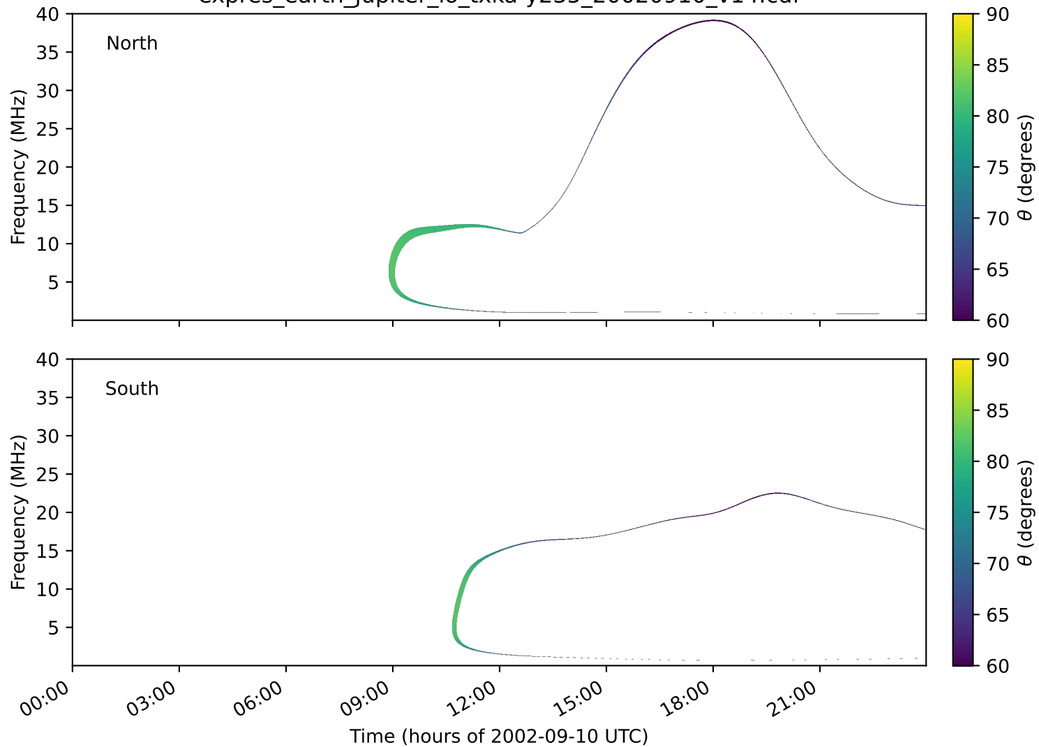
expres_earth_jupiter_io_txka-y235_20020910_v14.cdf
