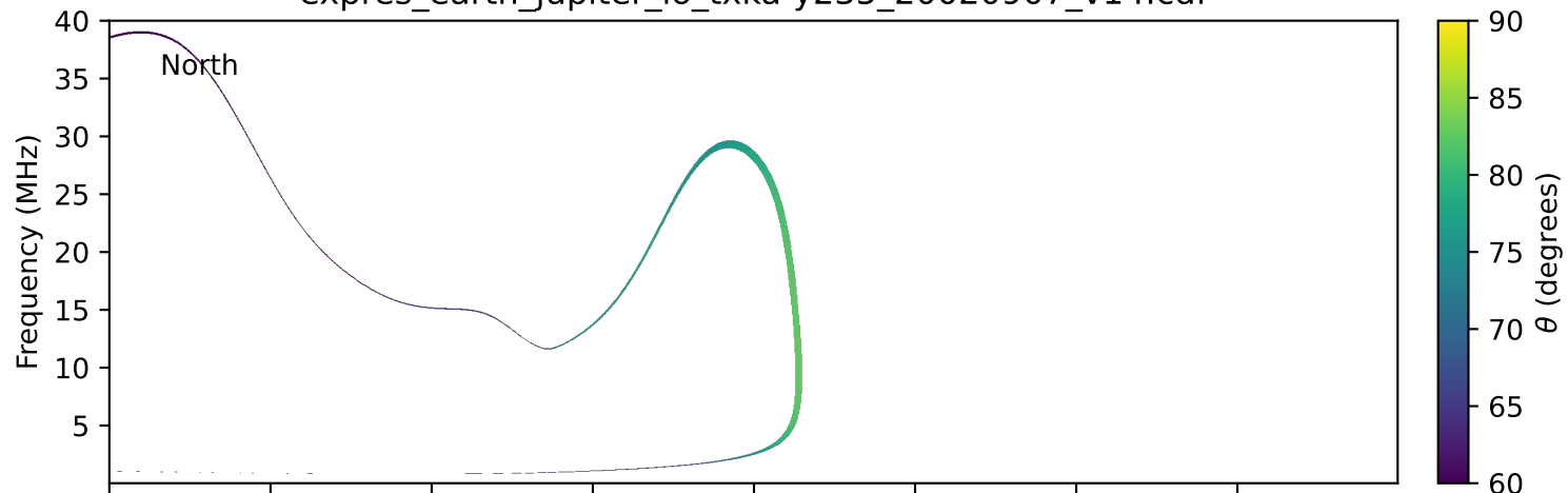
expres_earth_jupiter_io_txka-y235_20020907_v14.cdf
