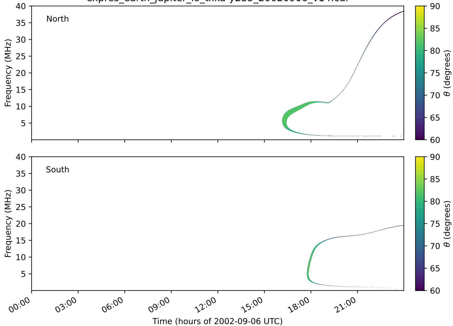
expres_earth_jupiter_io_txka-y235_20020906_v14.cdf
