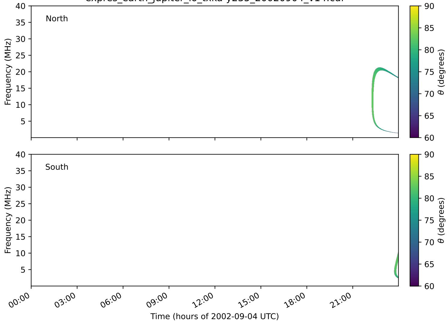
expres_earth_jupiter_io_txka-y235_20020904_v14.cdf
