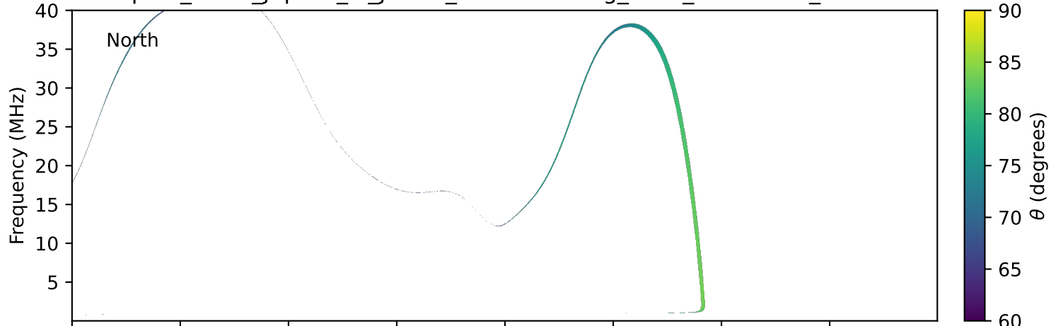
expres_earth_jupiter_io_jrm33_lossc-wid1deg_3kev_20020930_v11.cdf
