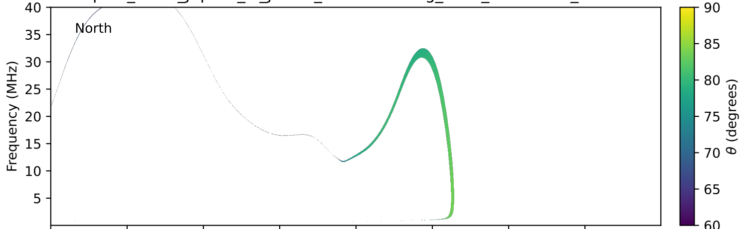
expres_earth_jupiter_io_jrm33_lossc-wid1deg_3kev_20020923_v11.cdf
