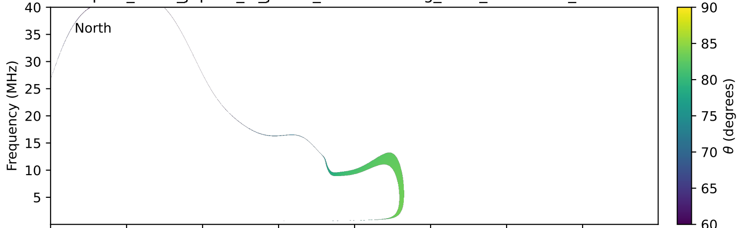
expres_earth_jupiter_io_jrm33_lossc-wid1deg_3kev_20020916_v11.cdf
