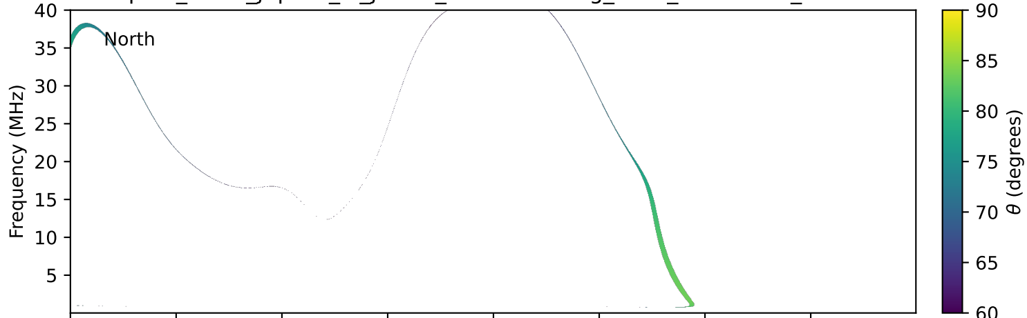
expres_earth_jupiter_io_jrm33_lossc-wid1deg_3kev_20020914_v11.cdf
