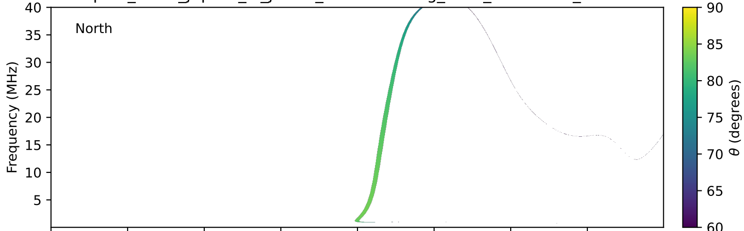
expres_earth_jupiter_io_jrm33_lossc-wid1deg_3kev_20020908_v11.cdf
