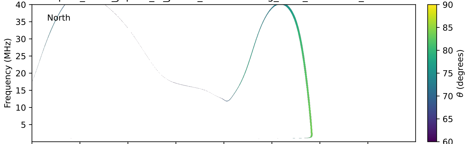
expres_earth_jupiter_io_jrm09_lossc-wid1deg_3kev_20020930_v11.cdf
