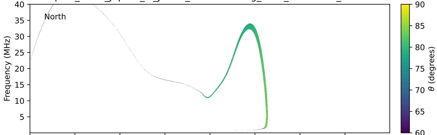
expres_earth_jupiter_io_jrm09_lossc-wid1deg_3kev_20020923_v11.cdf
