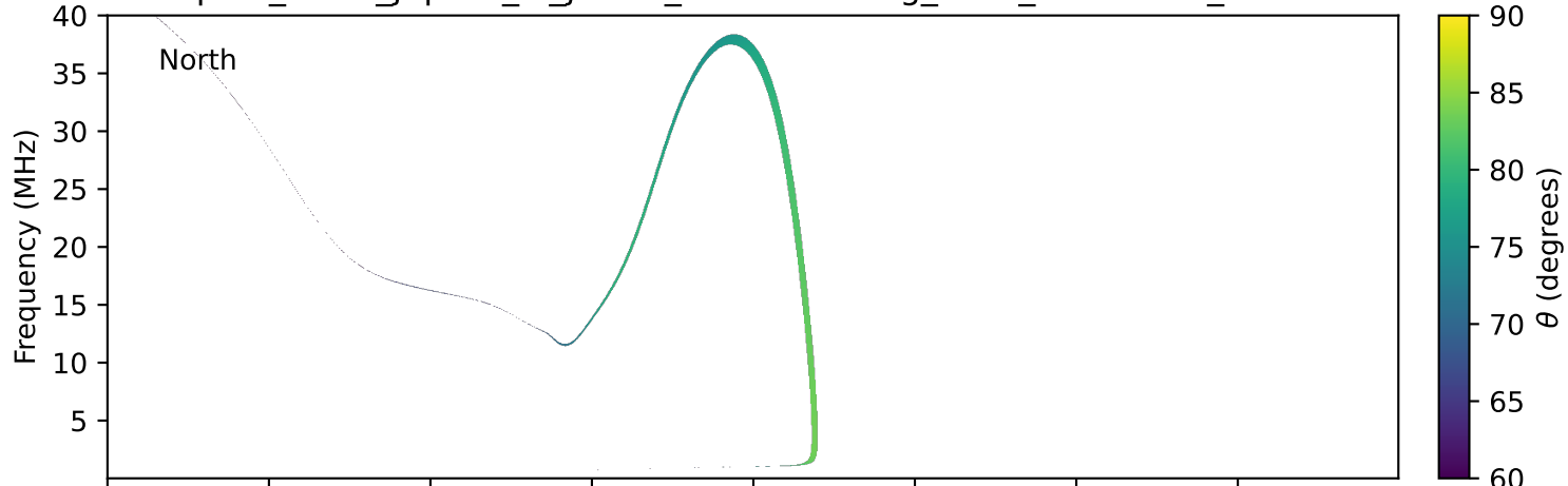
expres_earth_jupiter_io_jrm09_lossc-wid1deg_3kev_20020907_v11.cdf
