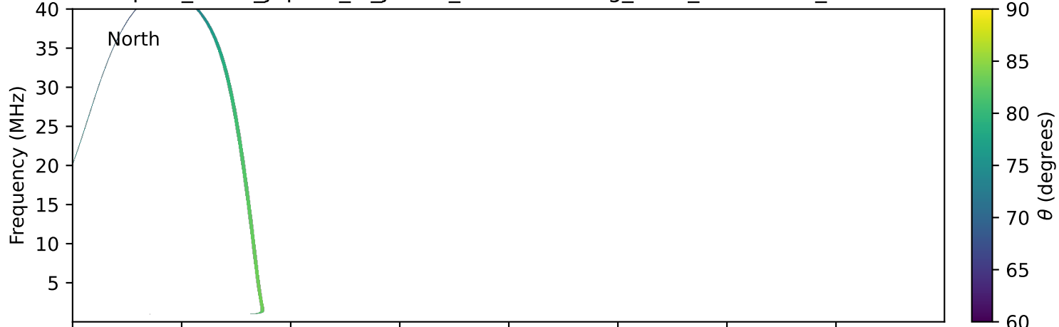
expres_earth_jupiter_io_jrm09_lossc-wid1deg_3kev_20020902_v11.cdf
